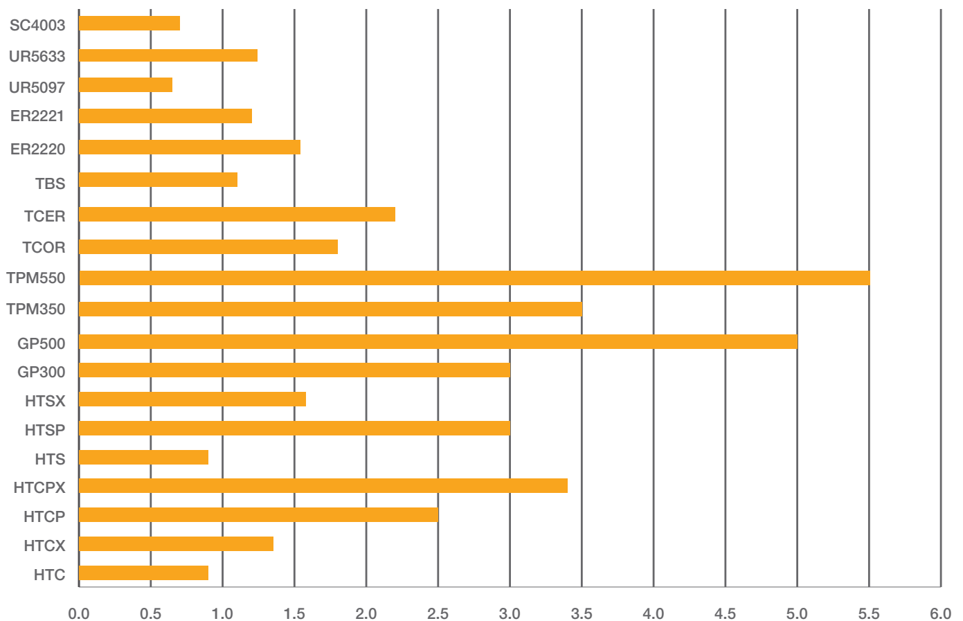
BULK THERMAL CONDUCTIVITY (W/m.K)
